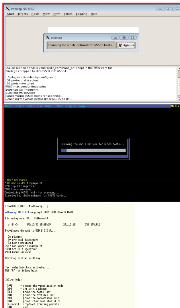
Interfaces Ettercap
