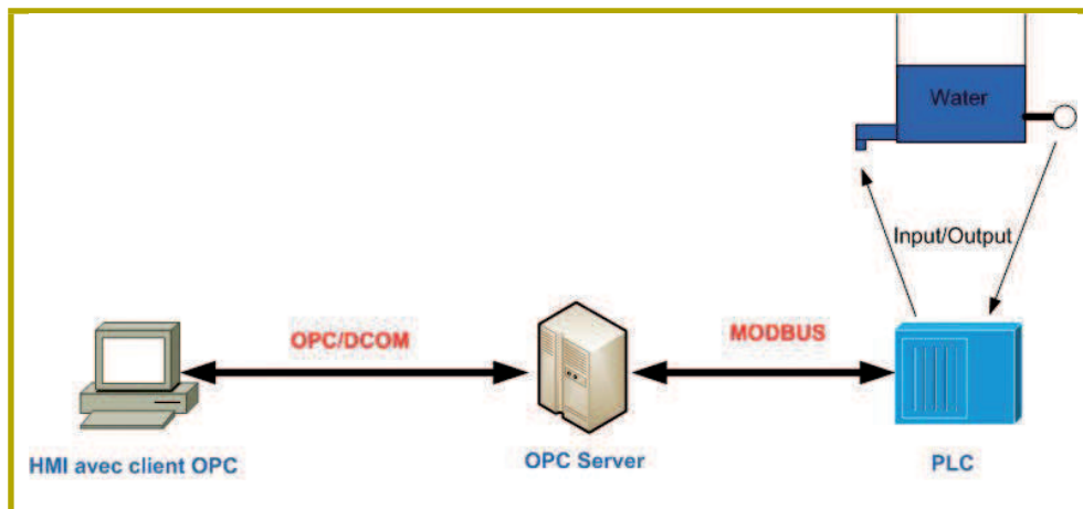
Figure 6 : SCADA network
