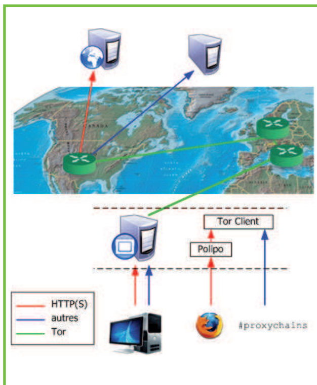
Figure 6 : ProxyChains + Tor
