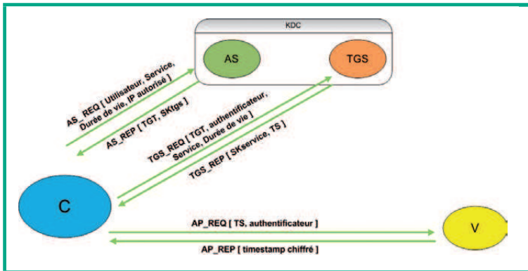
Kerberos Protocol
