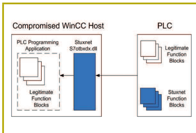
Figure 3 - Stuxnet
