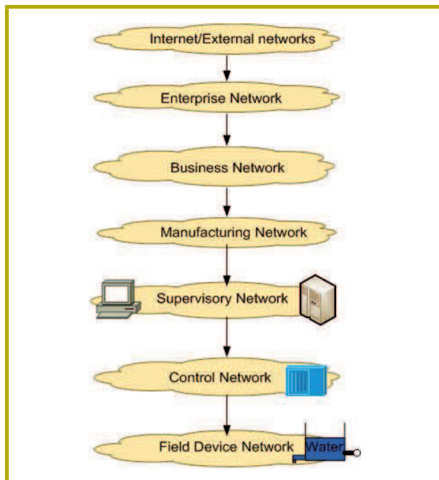
Figure 7 : Industrial System Network Segregation
