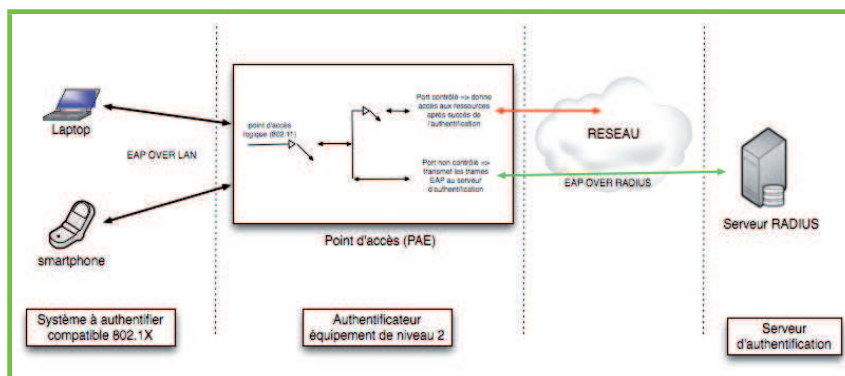
Figure 2 : Architecture d'authentification 802.1X
